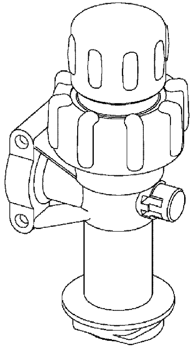
ASSEMBLY VIEW
