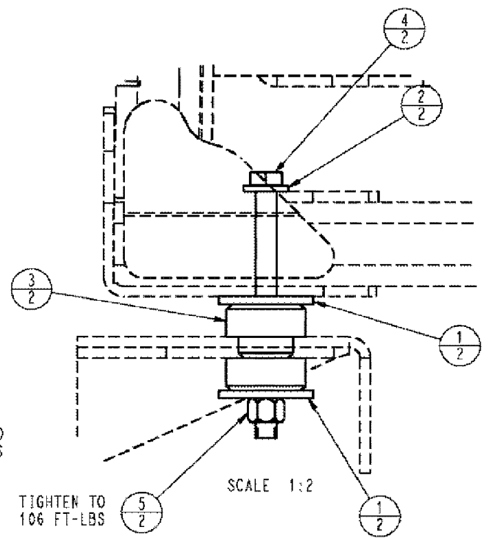
TYPICAL FRONT INSTALLATION
