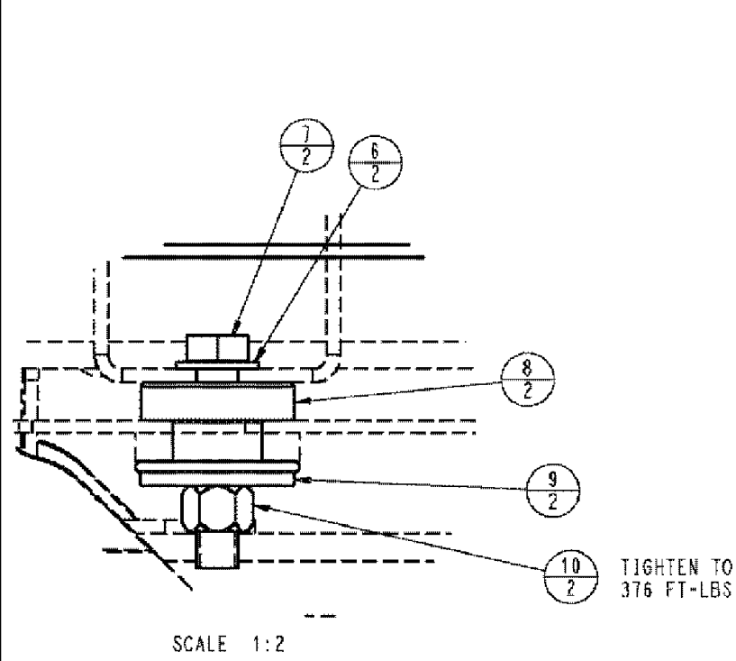
TYPICAL REAR INSTALLATION MOUNT IS SHOWN AFTER TAIL HAS BEEN FORMED
